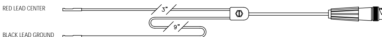
CABLE WITH .025" SQ SOCKETS P/N 9205 H/S
