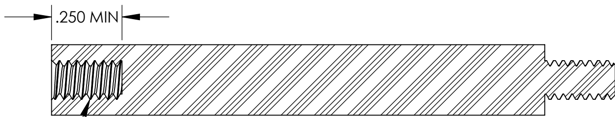
6-32 THREADS SECTION A-A
