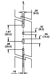
Mounting Style #1
