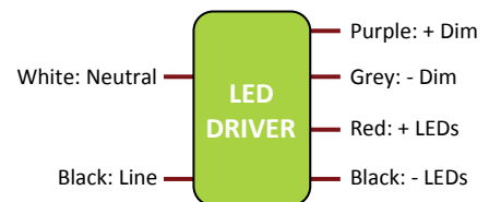
WIRING DIAGRAM
