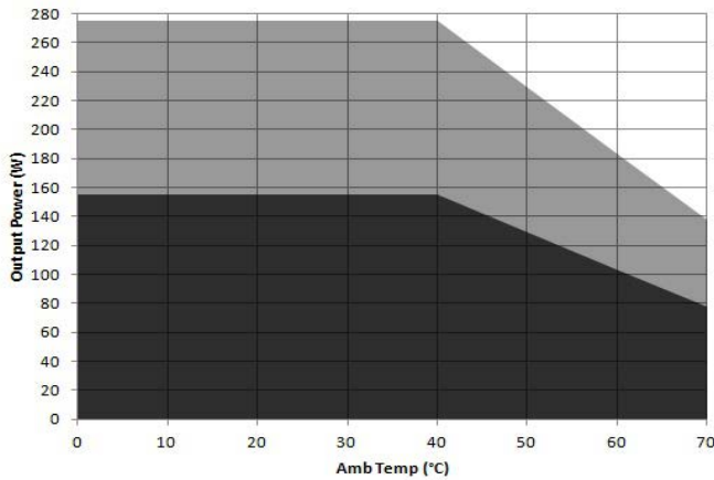
Power de-rating : 12V, 15V
