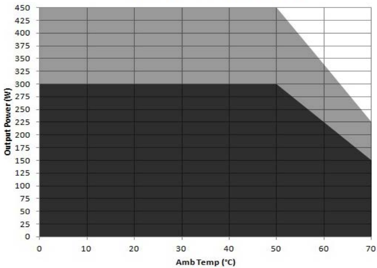
Power de-rating : 24V, 30V, 48V
