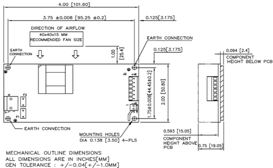
Input connector – Header Molex and Output Connector – Screw Terminal (Without PGPF)
