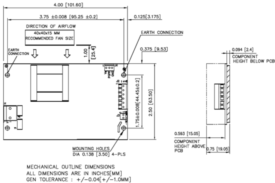
Input connector – Header Molex and Output Connector – Screw Terminal. (With PGPF)
