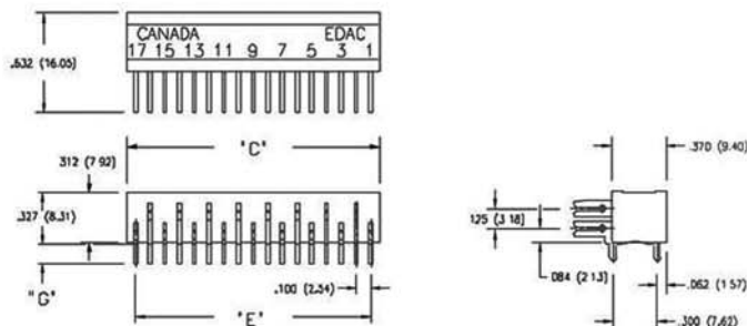
422 SERIES CONNECTOR
