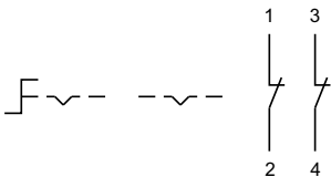
29 Selector switch 2 positions page 12 | Selector switch actuator 2 positions, flush mounting page 16
