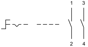
24 Selector switch 2 positions page 12 | Selector switch actuator 2 positions, flush mounting page 16
