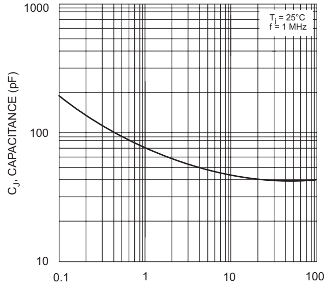
Fig. 4 Typ Junction Capacitance per element
