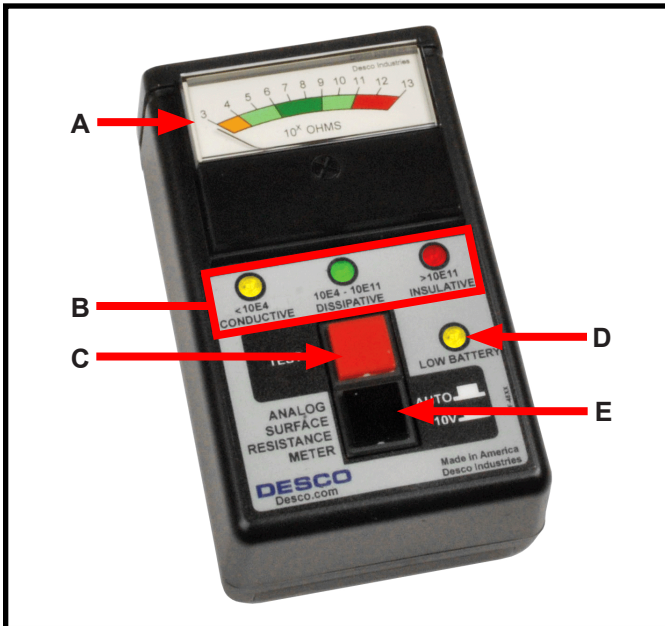
Figure 2. Analog Surface Resistance Meter features and components
