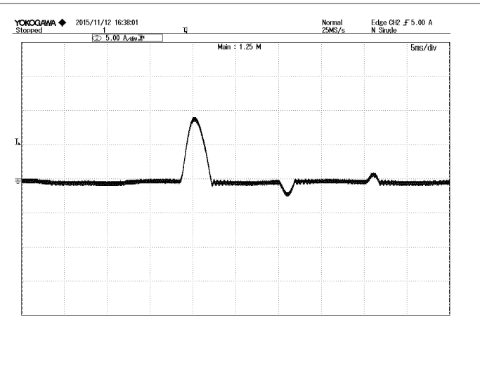
Figure 8: Inrush current @ Vin=220Vac lin: 5A/div, 5mS/div
