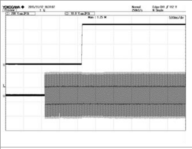
Figure 5: V_{out} start up at 220Vac, 10.5A I_{out} , TOP: VOUT, 10V/div, 500ms/div
