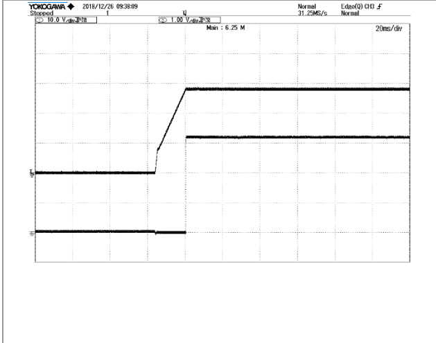
Figure 9: PG voltage vs. Vout @Vin=220Vac, 0Alout TOP: Vout, 10V/div, 20mS/div BOTTOM: PG, 1V/div, 20mS/div
