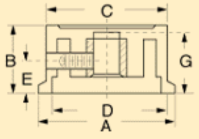
Brass Bushing w/ Set Screw
