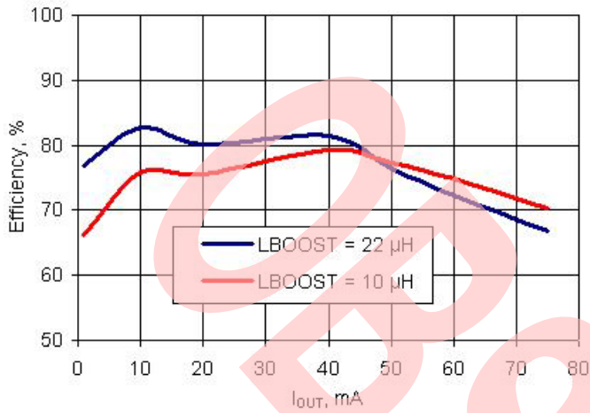
Figure 11-10. 效率与 I_{OUT} V_{BAT} = 2.4\text{ V} , V_{OUT} = 3.3\text{ V}
