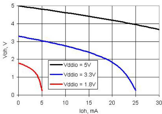
Figure 11-13. GPIO 输出高电压和电流
