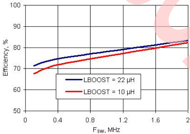
Figure 11-12. 效率与开关频率 V_{OUT} = 3.3\text{ V} , V_{BAT} = 2.4\text{ V} , I_{OUT} = 40\text{ mA}
