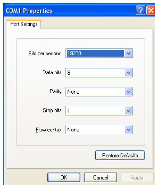
Figure 5-33. HyperTerminal Settings
