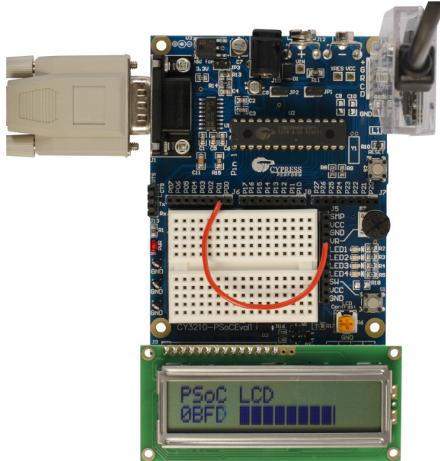
Figure 5-34. Verify Output on LCD
