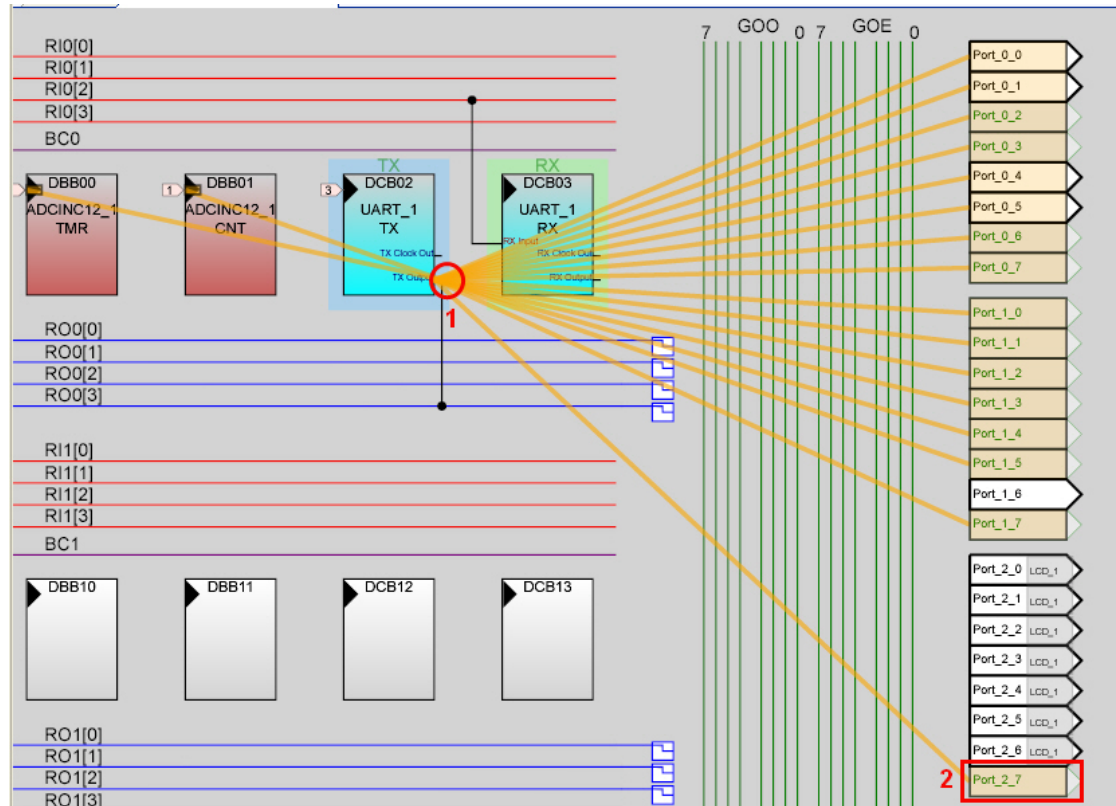
Figure 5-21. Auto-Routing
