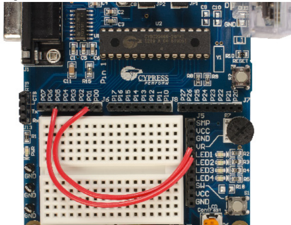
Figure 5-45. Hardware Connections: Code Example 4
