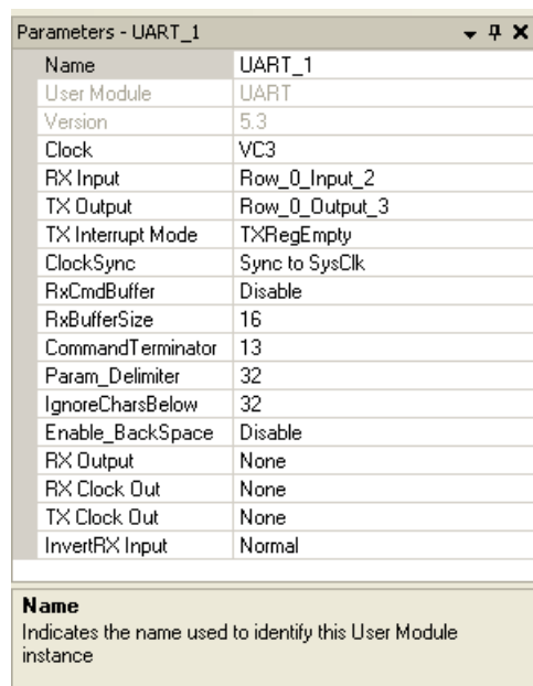
Figure 5-15. UART User Module Properties
