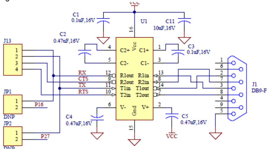
Figure 4-7. RS-232 Interface Schematic
