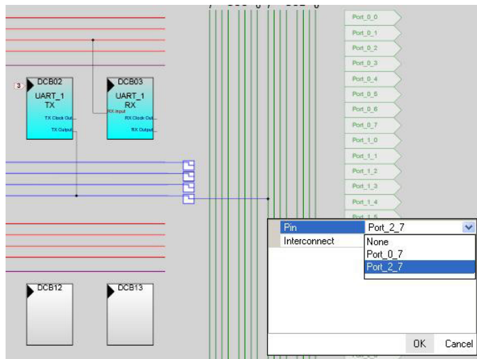
Figure 5-24. Pin Select
