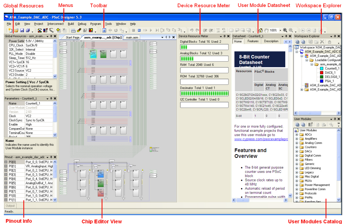
Figure 2-7. PSoC Designer Interconnect View
