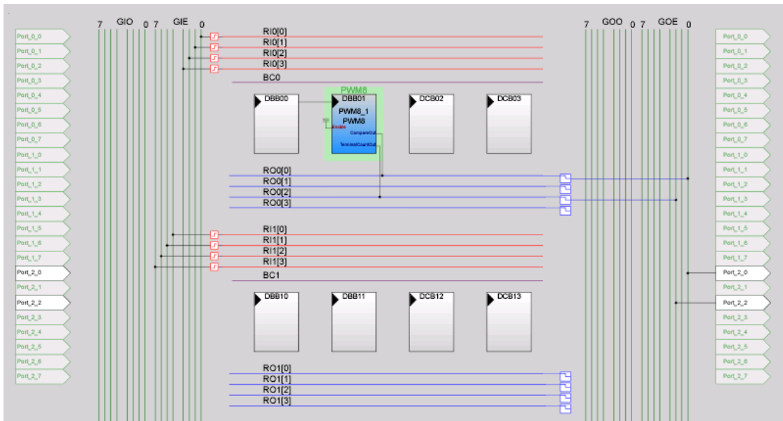
Figure 5-49. PWM Configuration
