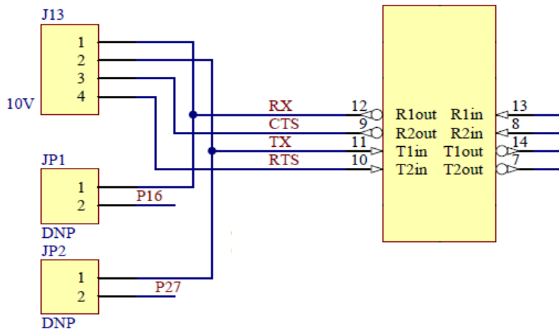
Figure 4-5. Jumper Settings
