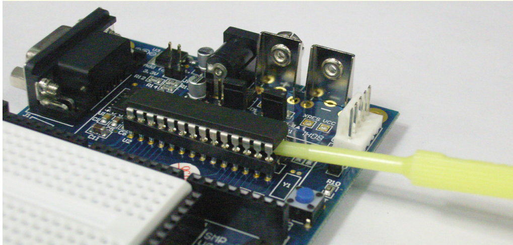
Figure A-4. Lift IC - One Side
