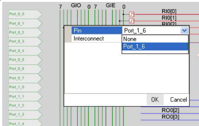
Figure 5-20. Pin Select
