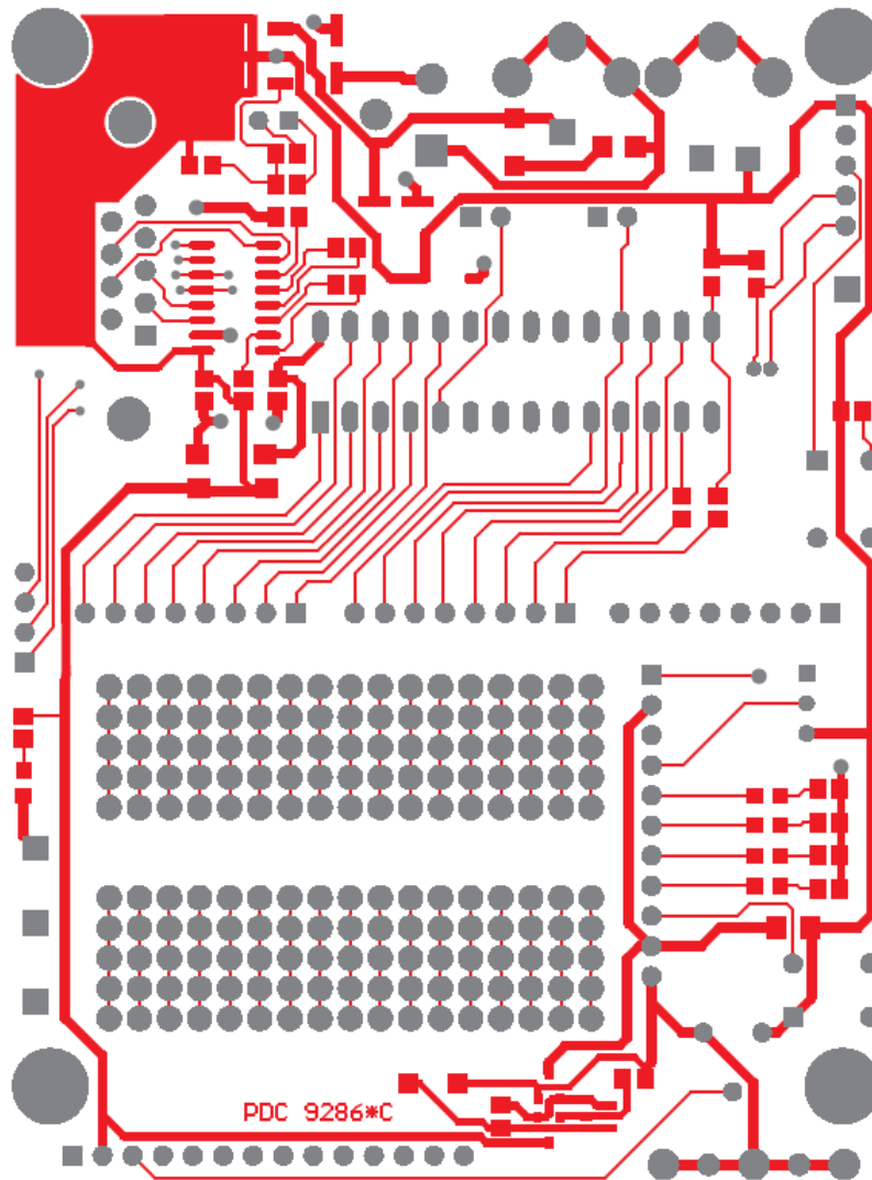
Figure A-1. Top Copper Layer
