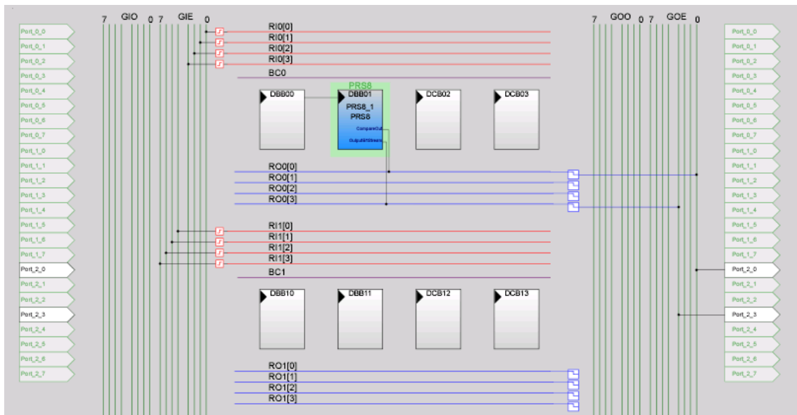
Figure 5-50. PRS Configuration
