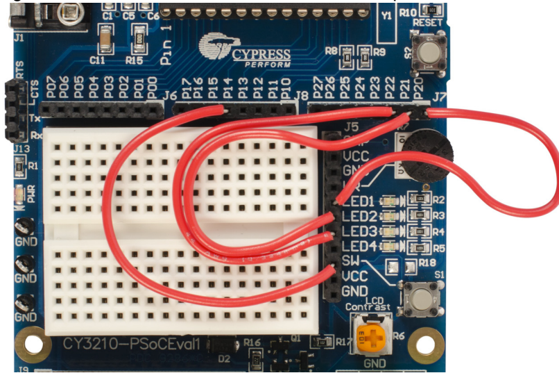
Figure 5-51. Hardware Connection: Code Example 5
