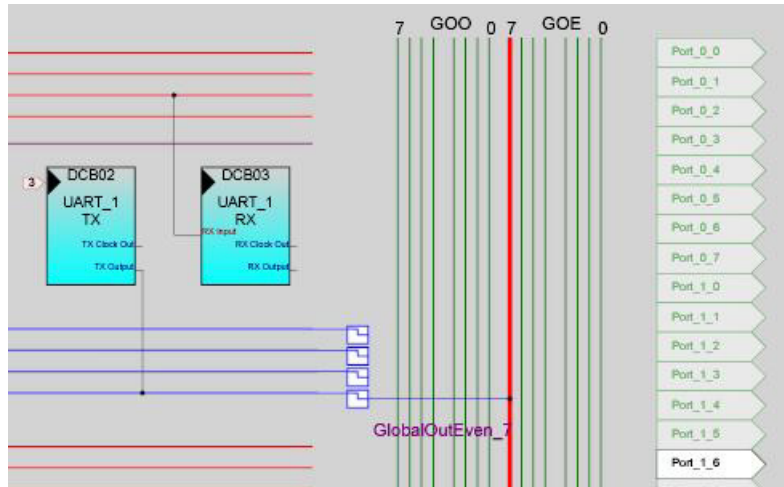
Figure 5-24. Pin Select
