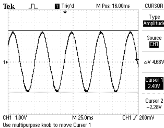
Figure 5-46. Output Sine Wave
