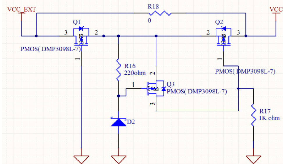
Figure 4-4. Protection Circuit
