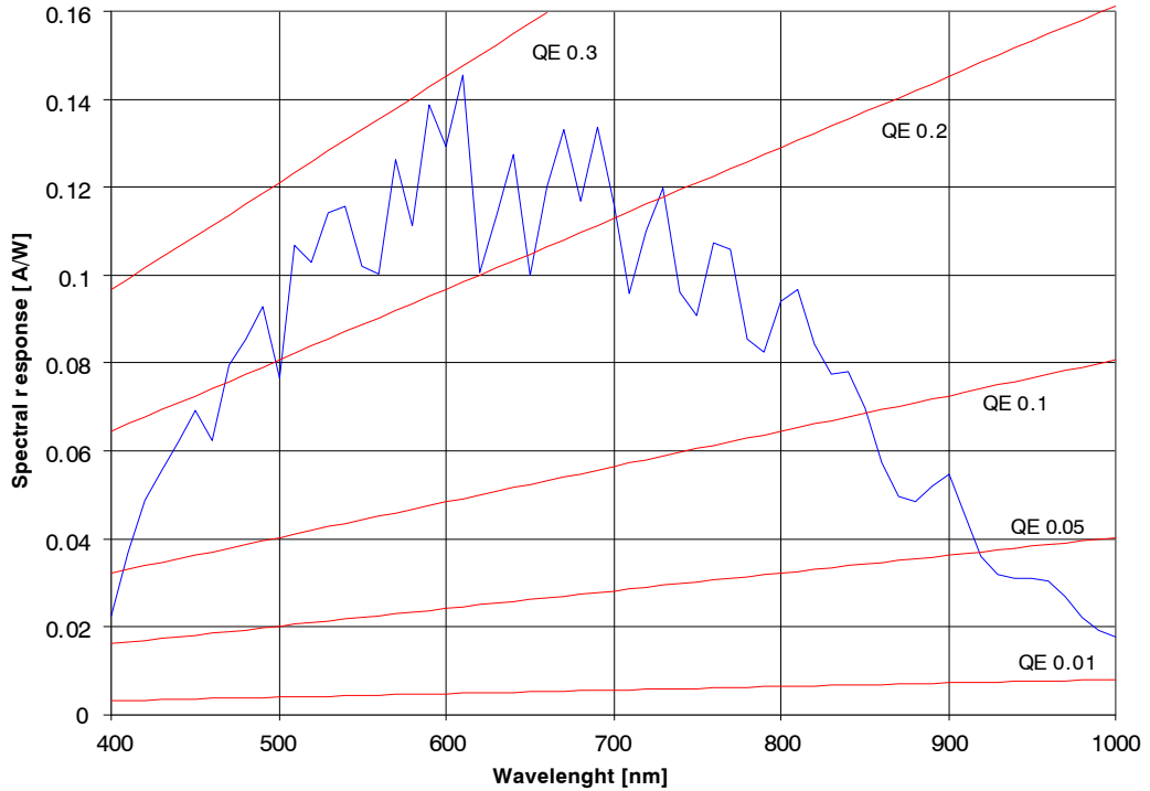
Figure 12. Spectral Response
