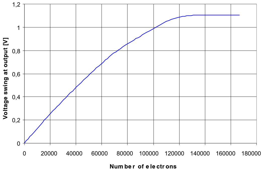
Figure 13. Photovoltaic Response
