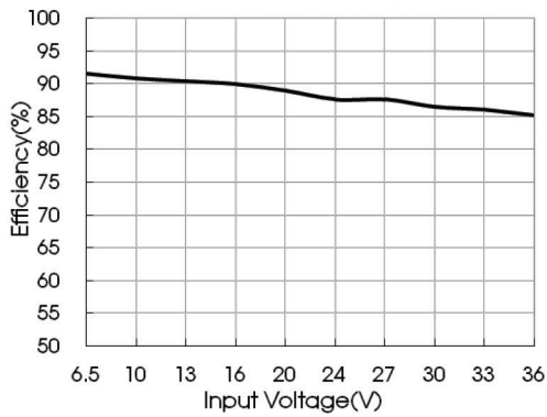
VX7805-500-W Efficiency Curve Efficiency vs. Input Voltage (at full load)
