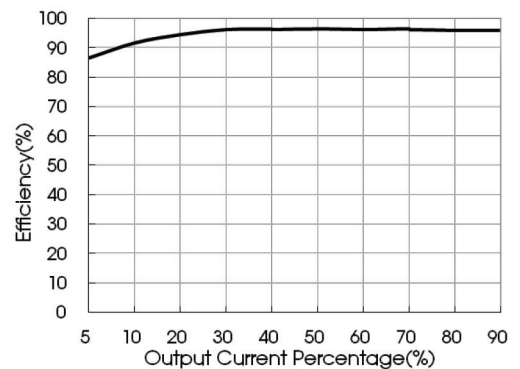
VX7815-500-W Efficiency Curve Efficiency vs. Output Load (Vin = 24V)
