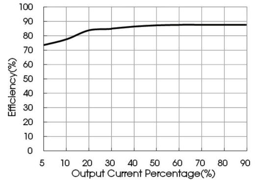
VX7805-500-W Efficiency Curve Efficiency vs. Output Load (Vin = 24V)
