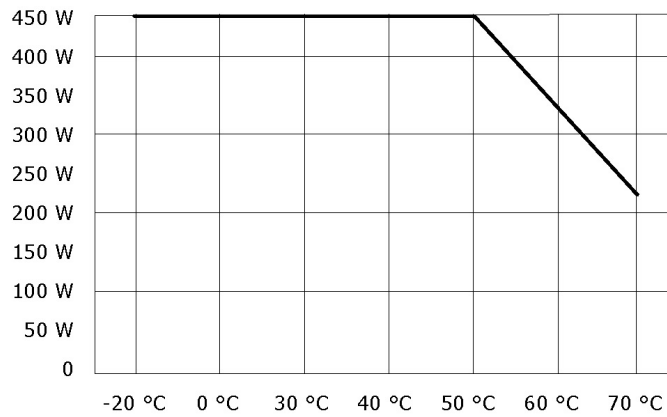
output power vs. ambient temperature
