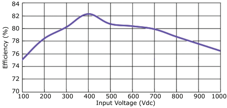
AE15-EW-S15-T Efficiency Curve Efficiency vs. Input Voltage
