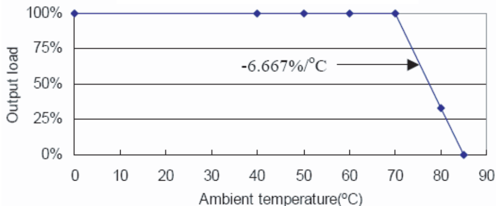
VOFM-5 series Derating Curve
