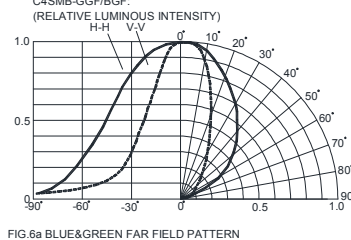
FIG.6a BLUE&GREEN FAR FIELD PATTERN
