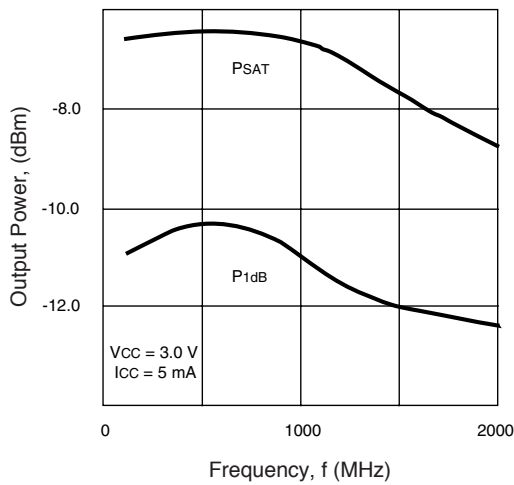
UPC2747TB POWER vs. FREQUENCY
