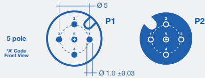
5 PINS A-CODED
