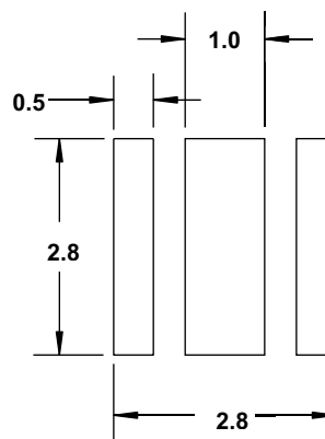
Figure 13: Recommended Soldering Land Pattern
