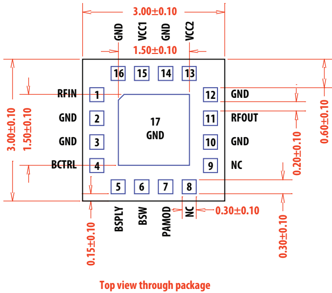
Figure 46. Package dimensions
