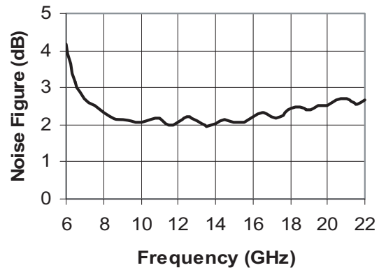
Figure 2b. Noise Figure
