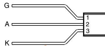
LP PACKAGE WITH FORMED LEADS (TOP VIEW)
