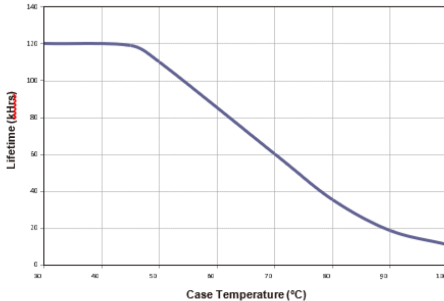
Lifetime vs Case Temperature
