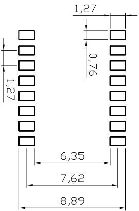
SMD SOLDERING PAD
