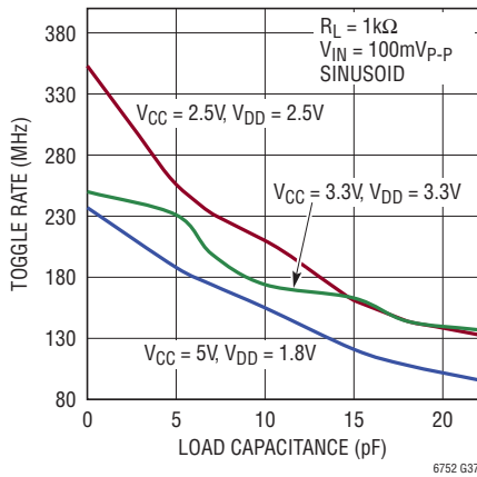
Toggle Rate vs Capacitive Load, LTC6752-3
