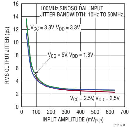
Output Jitter vs Input Amplitude
