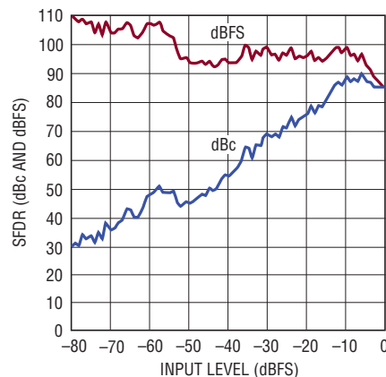
LTC2174-14: SFDR vs Input Level, f_{IN} = 70\text{MHz}, 2\text{V Range}, 105\text{Mpsps}
