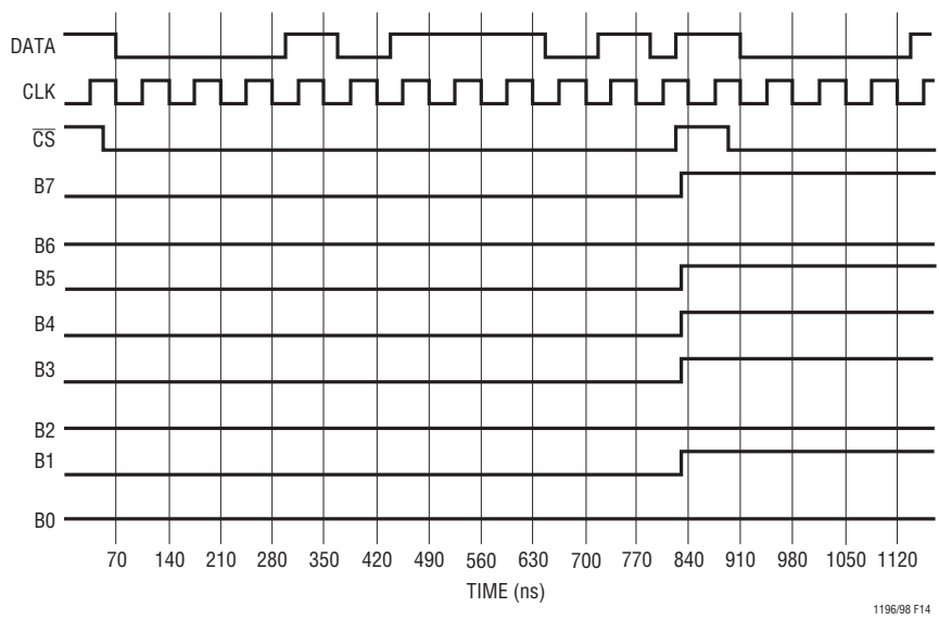
Figure 14. The Timing Diagram
