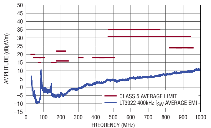
Average Radiated EMI Performance (CISPR25)
