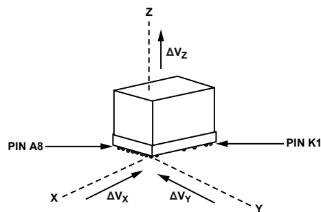
Figure 38. Delta Velocity Axis and Polarity Assignments
