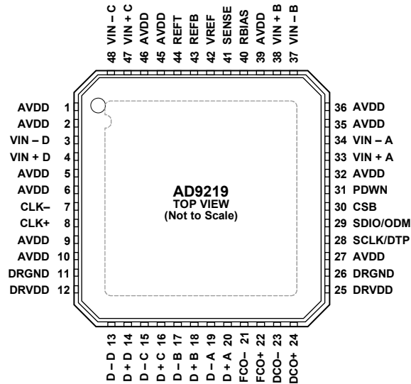
Figure 5. 48-Lead LFCSP Pin Configuration, Top View
