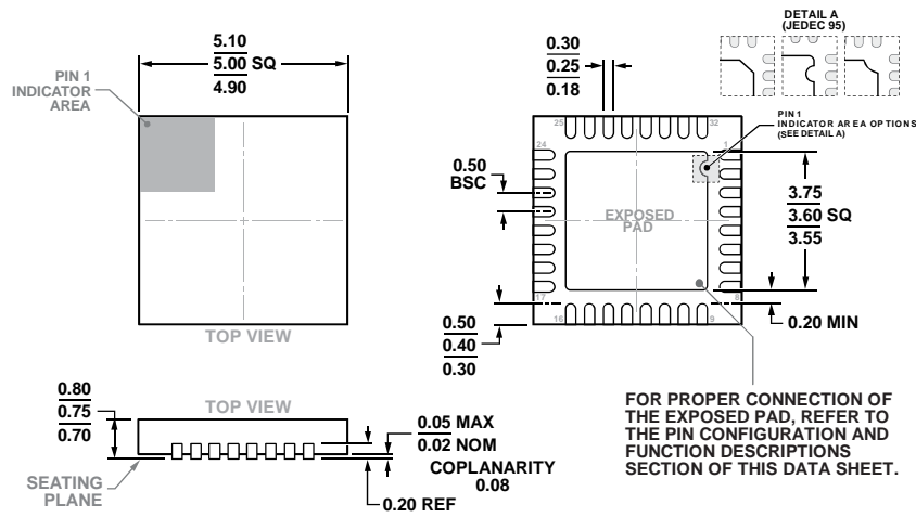
COMPLIANT TO JEDEC STANDARDS MO-220-WHHD-5 Figure 54. 32-Lead Lead Frame Chip Scale Package [LFCS] 5 mm × 5 mm Body and 0.75 mm Package Height (CP-32-12) Dimensions shown in millimeters
