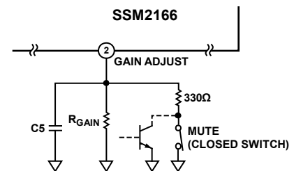
Figure 23. Details of Mute Option
