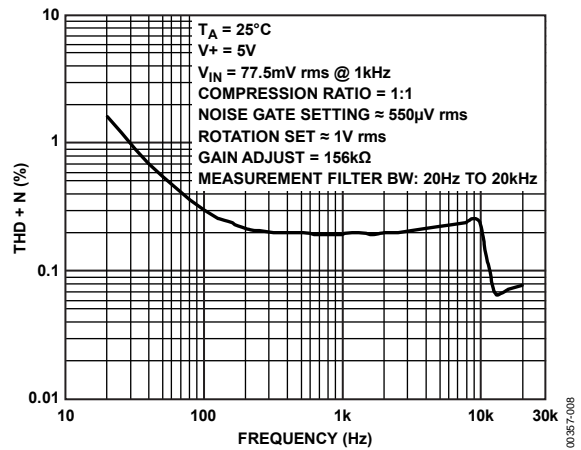
Figure 8. THD + N (%) vs. Frequency (Hz)
