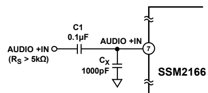
Figure 25. Circuit Configuration for Use with High Impedance Signal Sources
