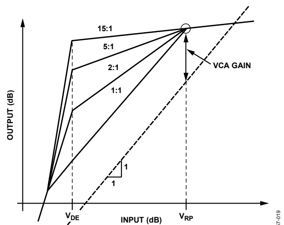
Figure 20. Effect of Varying the Compression Ratio
