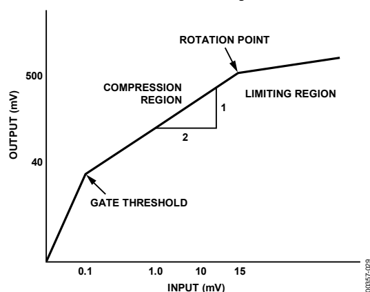
Figure 30. Transfer Characteristic
