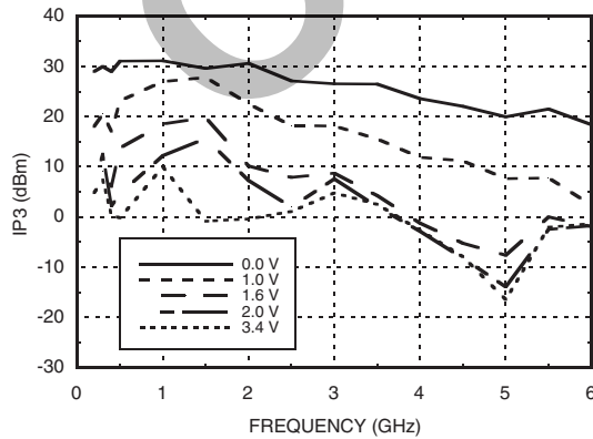
Output IP3 vs. Vctl [1]
