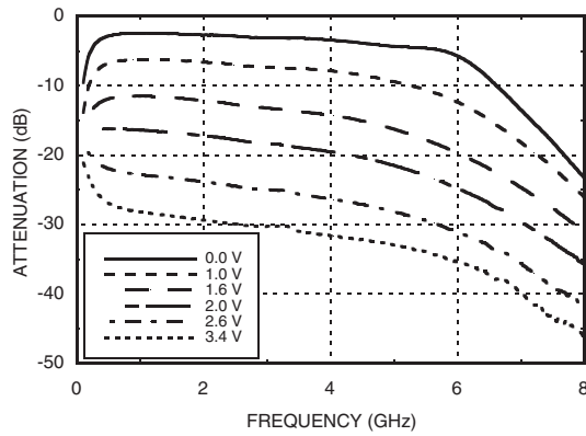
Insertion Loss vs. Vctl [2]
