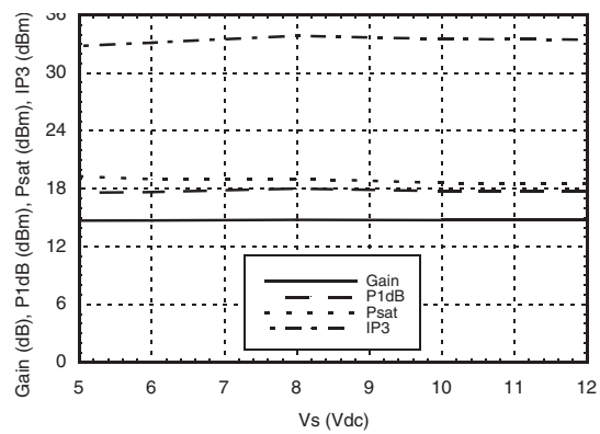
Gain, Power & OIP3 vs. Supply Voltage for Constant Icc= 72 mA @ 850 MHz
