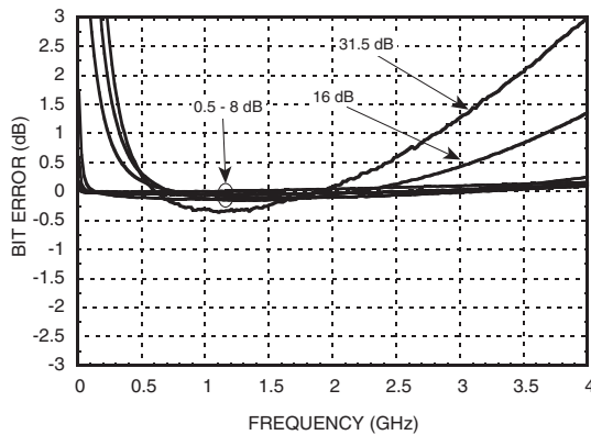
Bit Error vs. Frequency without AC Ground Caps
