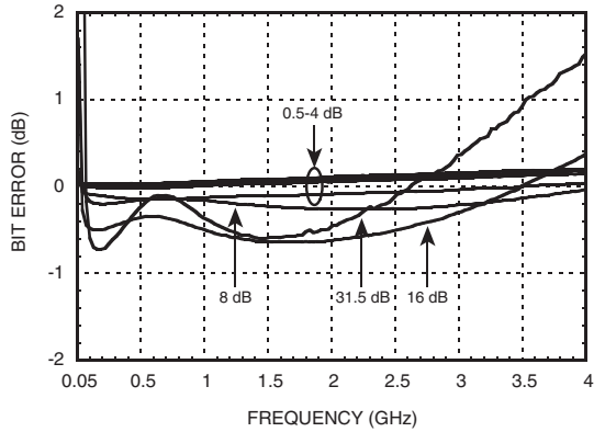
Bit Error vs. Frequency without AC Ground Caps
