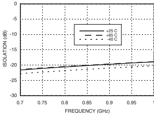
LNA Reverse Isolation vs. Temperature
