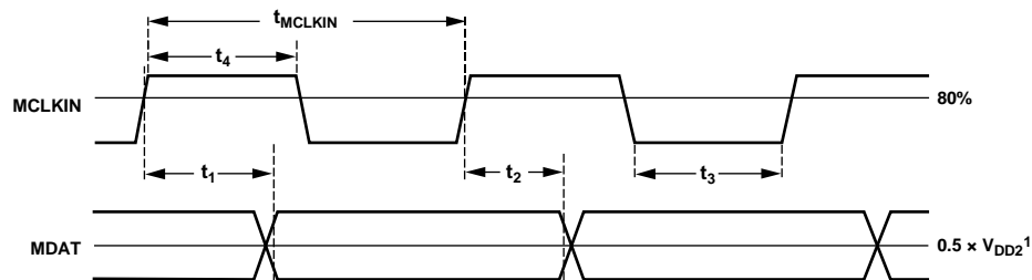
Figure 2. Data Timing Diagram
