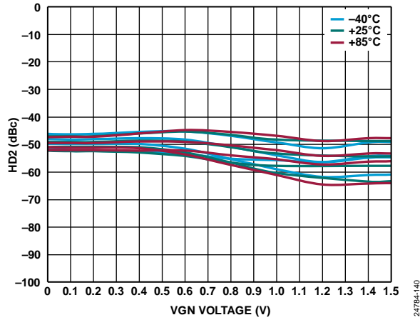
Figure 39. HD2 vs. VGN Voltage over Temperature and OFSx at 3 GHz
