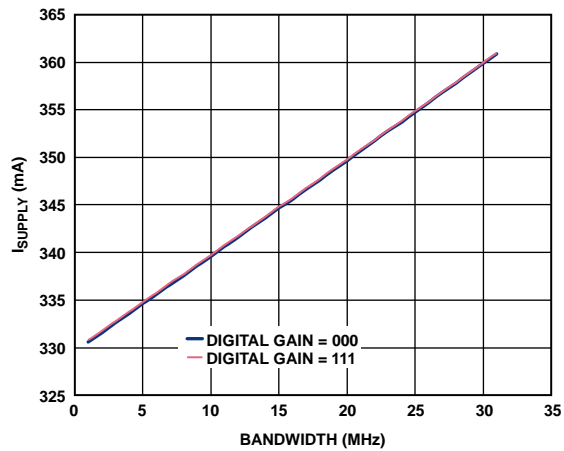
Figure 40. Current Consumption at Minimum and Maximum Digital Gain vs. Bandwidth (Bandwidth Setting = 31 MHz, Gain = 30 dB)
