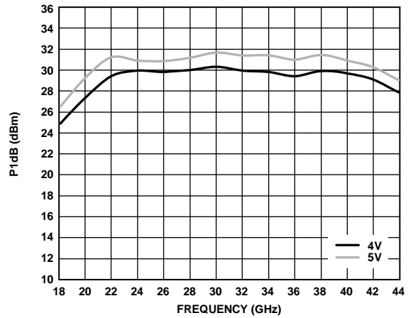
Figure 25. P1dB vs. Frequency for Various Supply Voltages, I_{DQ} = 1400\text{ mA}
