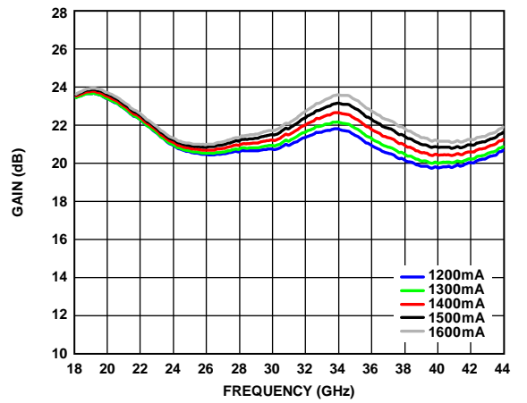
Figure 14. Gain vs. Frequency for Various Supply Currents, V_{DD} = 5\text{ V}
