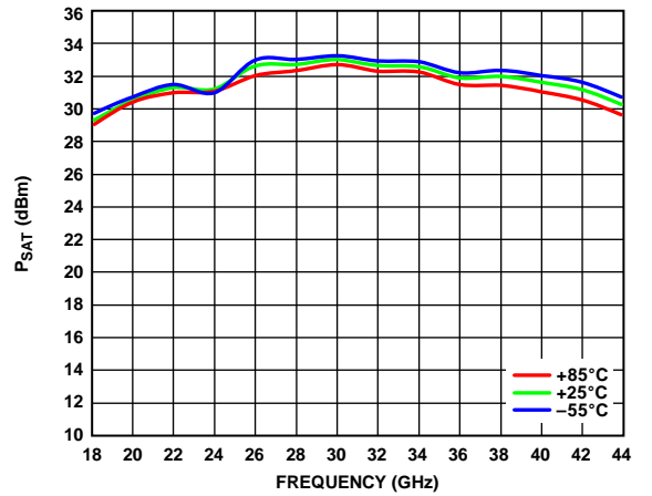
Figure 26. P_{SAT} vs. Frequency for Various Temperatures, V_{DD} = 5V, I_{DQ} = 1400\text{ mA}
