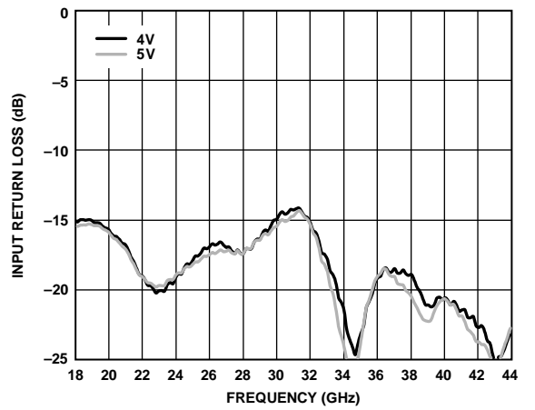
Figure 15. Input Return Loss vs. Frequency for Various Supply Voltages, I_{DQ} = 1400\text{ mA}
