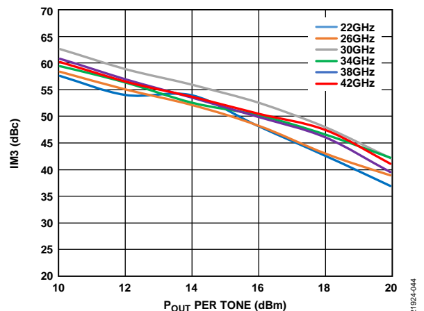
Figure 44. IM3 Distortion Relative to Carrier vs. P_{OUT} per Tone, V_{DD} = 5 V, I_{DQ} = 1400 mA
