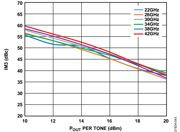
Figure 43. IM3 Distortion Relative to Carrier vs. P_{OUT} per Tone, V_{DD} = 4 V, I_{DQ} = 1400 mA
