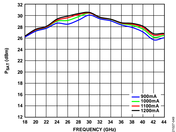
Figure 49. P SAT vs. Frequency for Various Drain Currents, V DD = 5 V, Data Measured with Constant I DD
