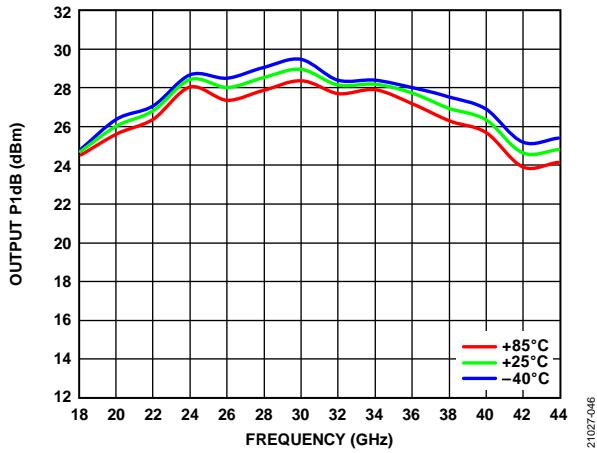
Figure 46. Output P1dB vs. Frequency for Various Temperatures, V DD = 5 V, Data Measured with Constant I DD
