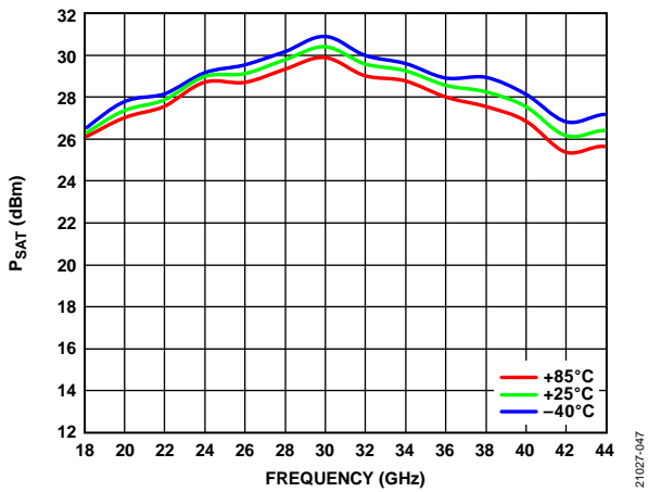
Figure 47. P SAT vs. Frequency for Various Temperatures, V DD = 5 V, Data Measured with Constant I DD
