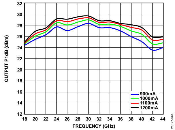
Figure 48. Output P1dB vs. Frequency for Various Drain Currents, V DD = 5 V, Data Measured with Constant I DD
