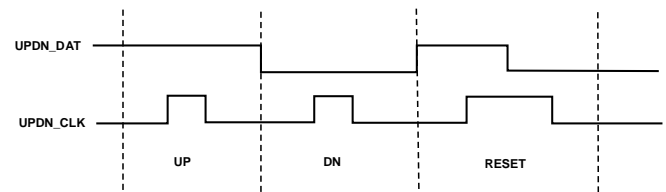
Figure 3. UP/DOWN Timing
