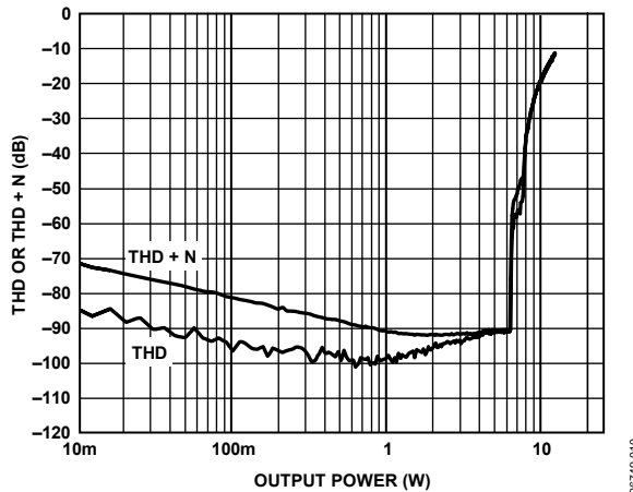
Figure 11. THD or THD + N vs. Output Power, 8 Ω, PVDD = 12 V
