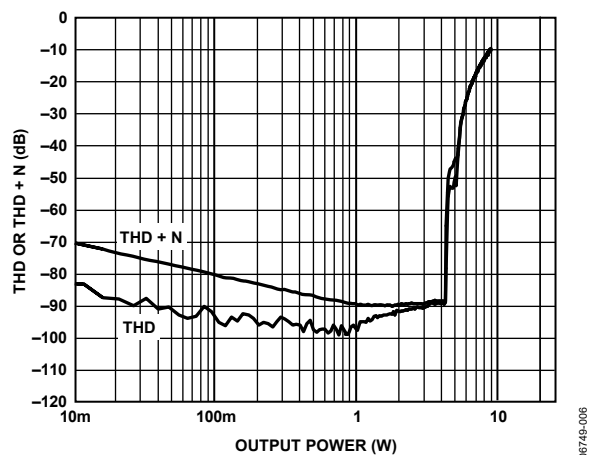
Figure 7. THD or THD + N vs. Output Power, 6 Ω, PVDD = 9 V
