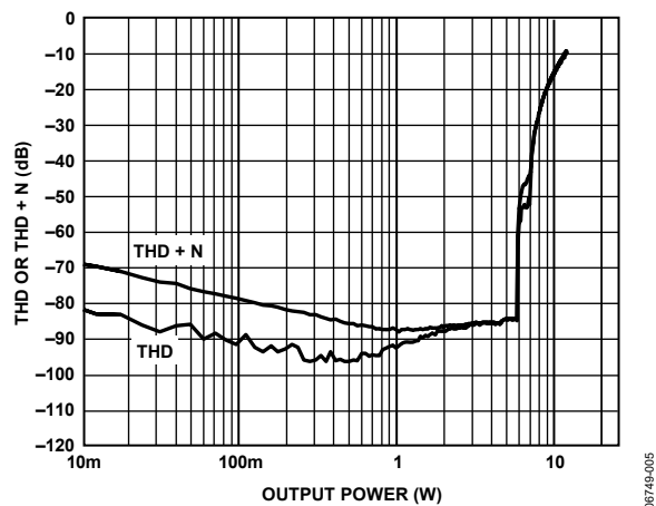
Figure 6. THD or THD + N vs. Output Power, 4 Ω, PVDD = 9 V
