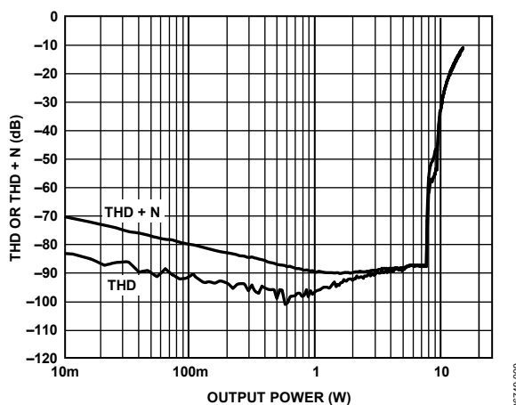
Figure 10. THD or THD + N vs. Output Power, 6 Ω, PVDD = 12 V
