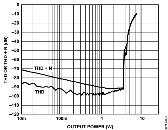
Figure 8. THD or THD + N vs. Output Power, 8 Ω, PVDD = 9 V
