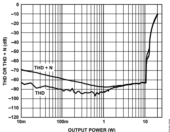
Figure 9. THD or THD + N vs. Output Power, 4 Ω, PVDD = 12 V
