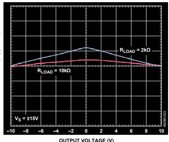
Figure 21. Gain Nonlinearity, G = 10
