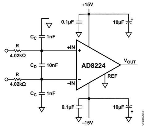
Figure 61. RFI Suppression
