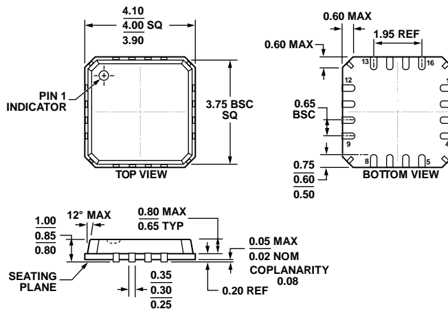
Figure 68. 16-Lead Lead Frame Chip Scale Package [LFCSP_VQ] 4 mm × 4 mm Body, Very Thin Quad, with Hidden Paddle (CP-16-19) Dimensions shown in millimeters
