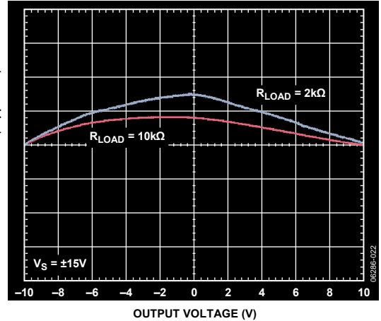
Figure 20. Gain Nonlinearity, G = 1
