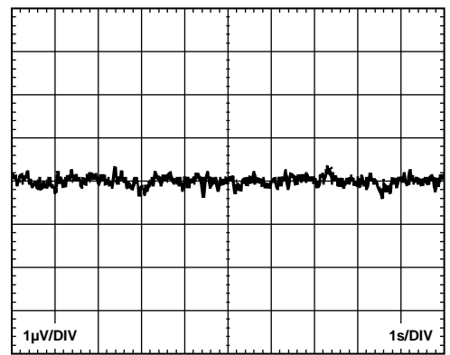
Figure 8. 0.1 Hz to 10 Hz RTI Voltage Noise (G = 1)
