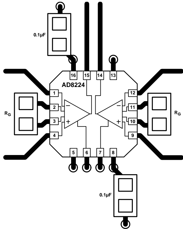
Figure 58. Example Layout
