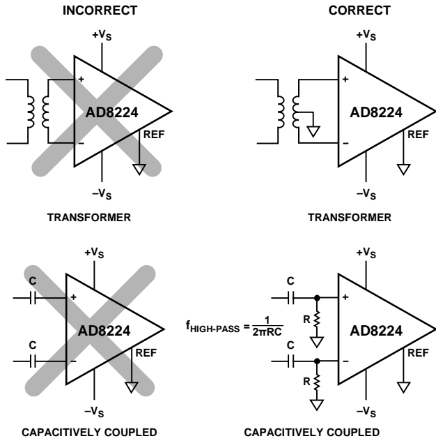
Figure 59. Creating an IBIAS Path
