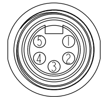
Conn. 1&3 Pin Assignments Front View
