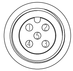
Conn.1&2&3&4&5 Pin Assignments Front View
