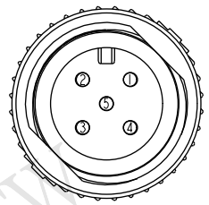
Conn.6 Pin Assignments Front View
